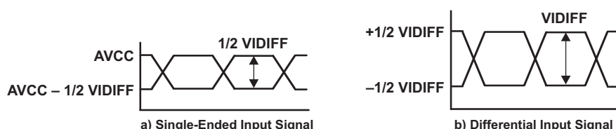
Figure 16. TMDS Inputs
