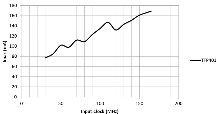
Figure 1. I_{max} vs Input Frequency
