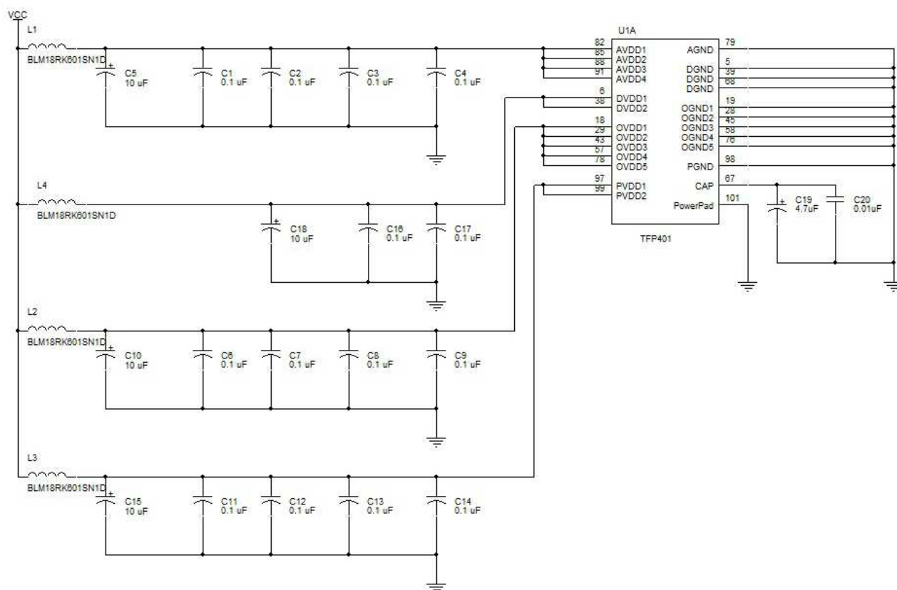
Figure 21. Power Supplies Decoupling Design
