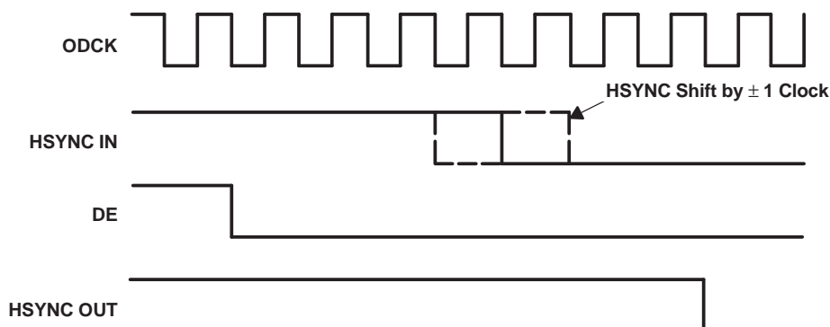
Figure 17. HSYNC Regeneration Timing Diagram
