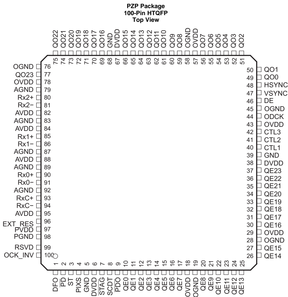
Pin Functions
