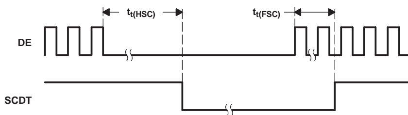
Figure 13. Time Between DE Transitions to SCDT Low and SCDT High
