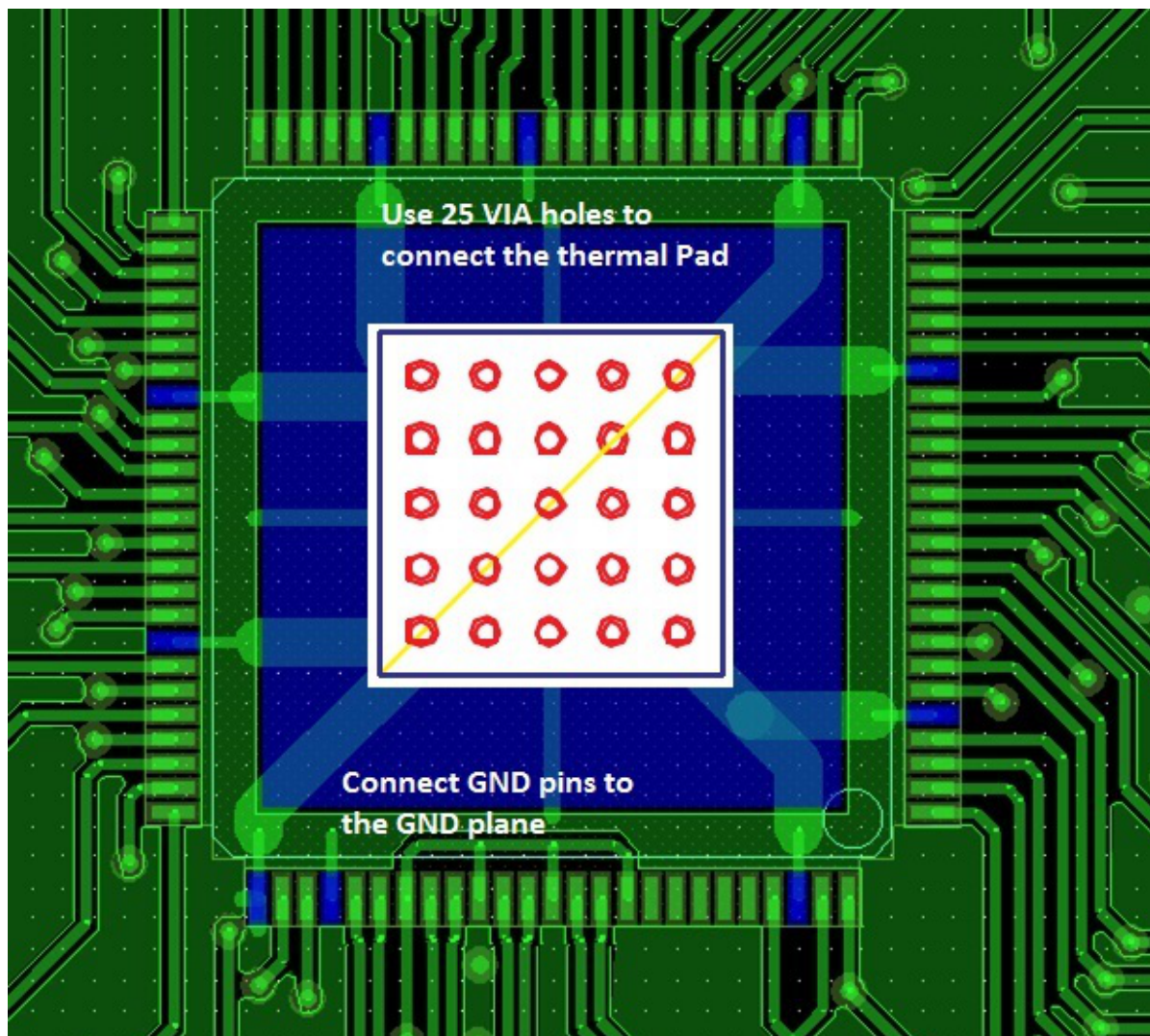
Figure 27. Ground Routing
