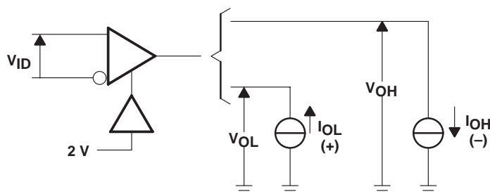
Figure 1. V_{OH} , V_{OL}
