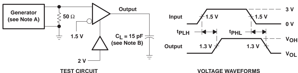
TEST CIRCUIT
