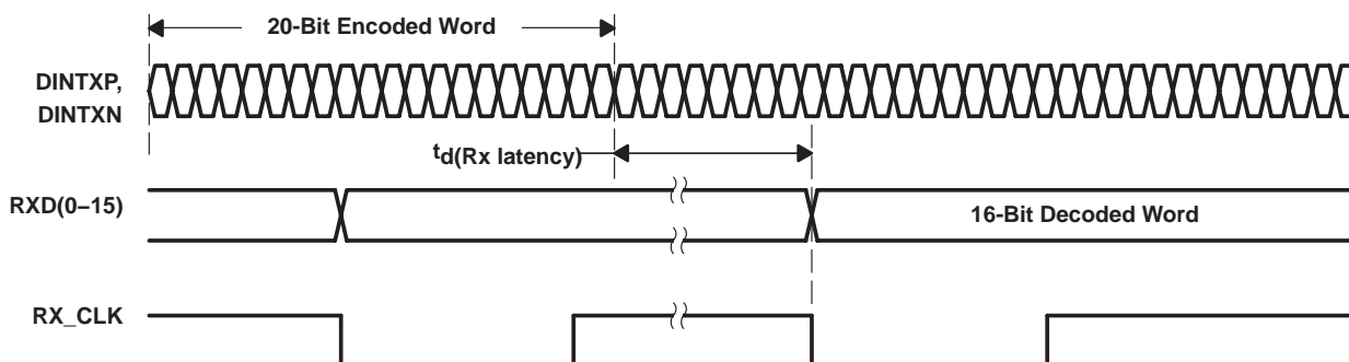
Figure 5. Receiver Latency
