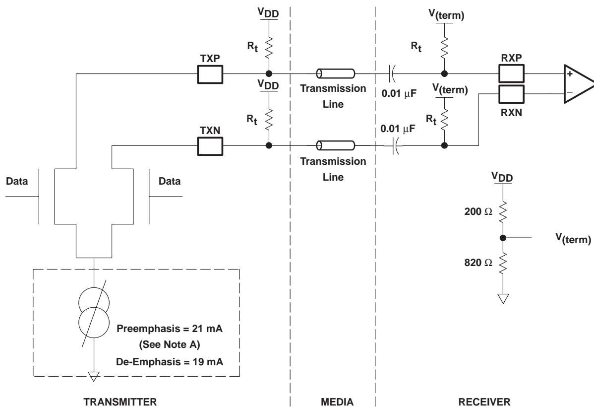
Figure 16. High-Speed I/O AC-Coupled Mode
