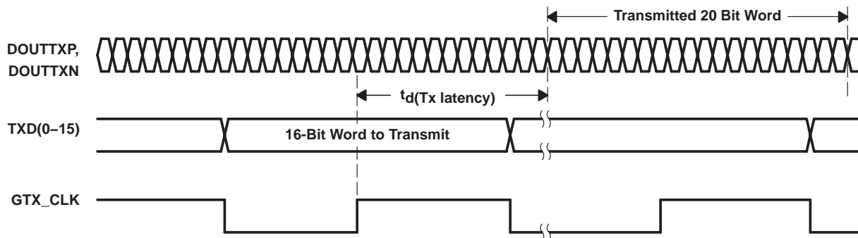
Figure 3. Transmitter Latency
