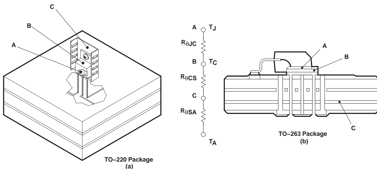
Figure 21. Thermal Resistances
