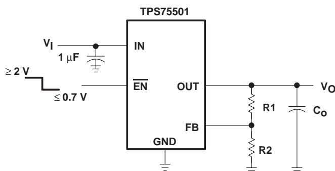
Figure 28. TPS75501 Adjustable LDO Regulator Programming
