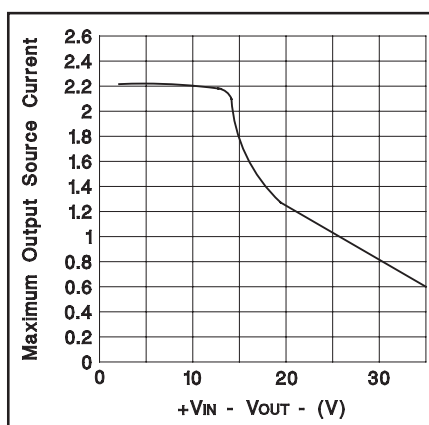
Maximum source current vs. +V_{IN} - V_{\text{OUT}} .
