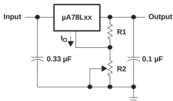
Figure 3. Adjustable-Output Regulator
