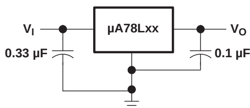
Figure 1. Fixed-Output Regulator
