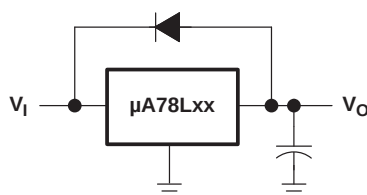
Figure 7. Reverse-Bias-Protection Circuit
