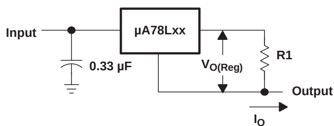
Figure 4. Current Regulator
