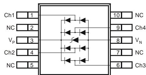
Device Schematic
