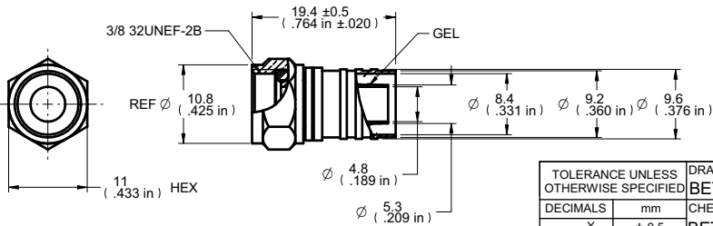
DIM OUTLINE
