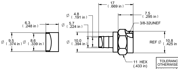
DIM OUTLINE
