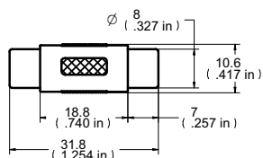
DIM OUTLINE
