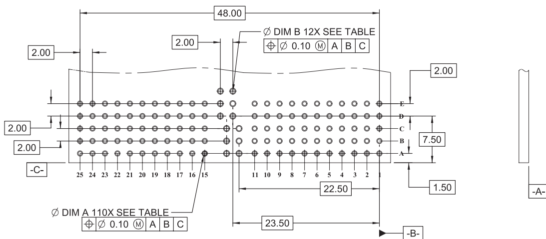
Recommended PCB hole mounting pattern
