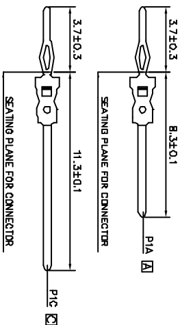
CONTACT DIMENSION
