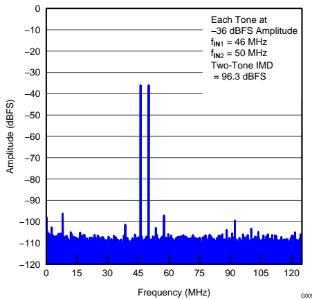
Figure 5. Two-Tone Input Signal
