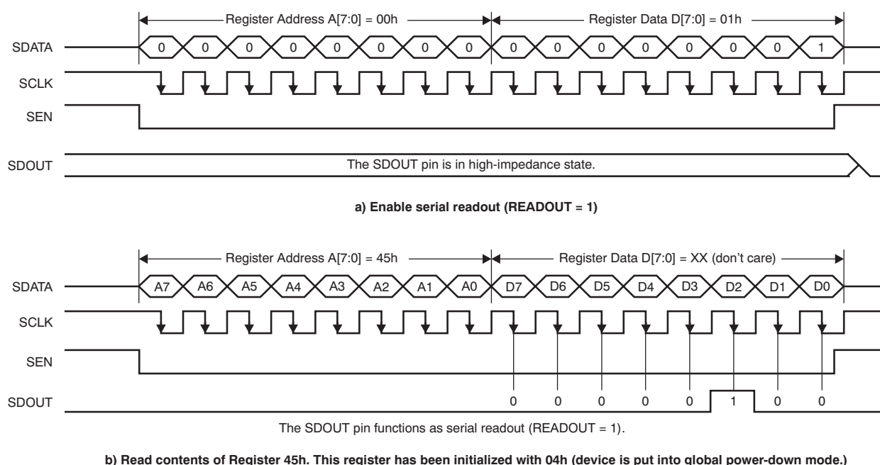
Figure 52. Serial Readout Timing Diagram
