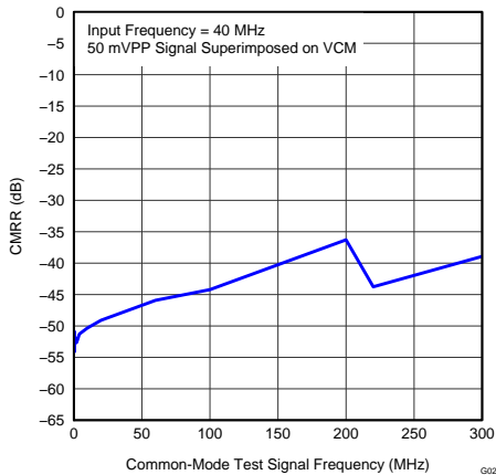
Figure 27. Common-Mode Rejection Ratio vs Test Signal Frequency
