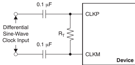
Figure 57. Differential Sine-Wave Clock Driving Circuit
