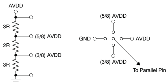
Figure 49. Simple Scheme to Configure the Parallel Pins
