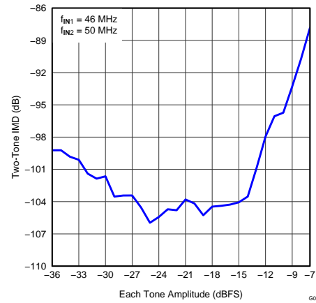
Figure 8. Two-Tone IMD3 vs Input Amplitude
