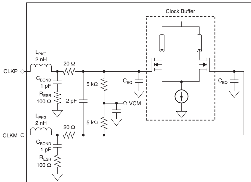
Figure 60. Internal Clock Buffer
