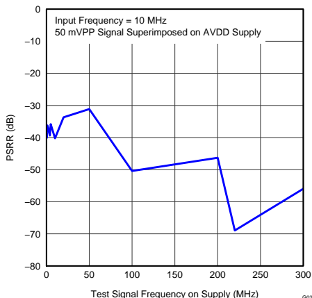
Figure 29. Power-Supply Rejection Ratio vs Test Signal Frequency
