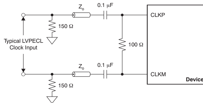
Figure 59. LVPECL Clock Driving Circuit
