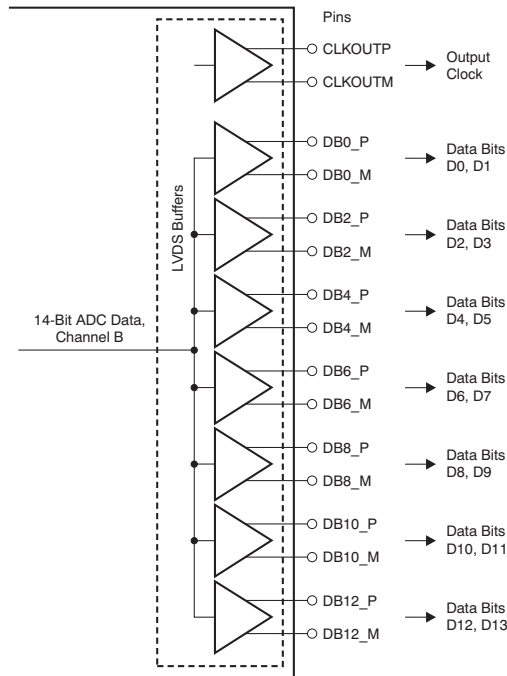
Figure 43. LVDS Interface
