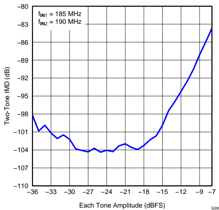
Figure 9. Two-Tone IMD3 vs Input Amplitude
