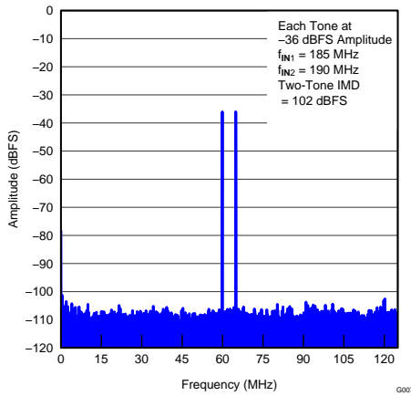
Figure 7. Two-Tone Input Signal
