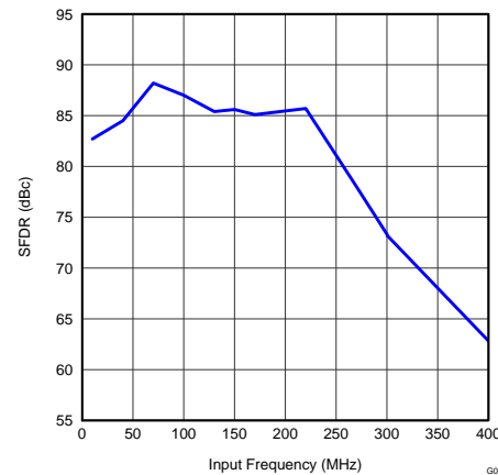
Figure 10. Spurious-Free Dynamic Range vs Input Frequency
