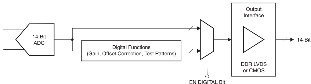
Figure 42. Digital Processing Block
