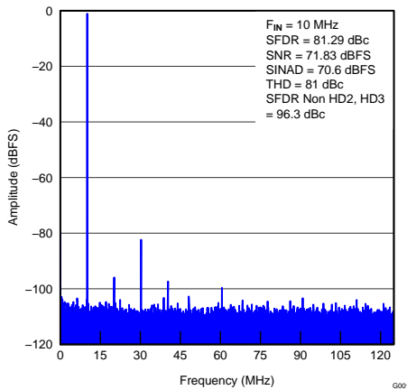
Figure 1. Input Signal (10 MHz)
