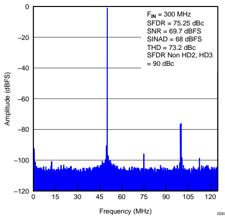
Figure 3. Input Signal (300 MHz)
