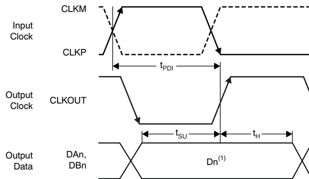
Figure 39. CMOS Interface Timing Diagram
