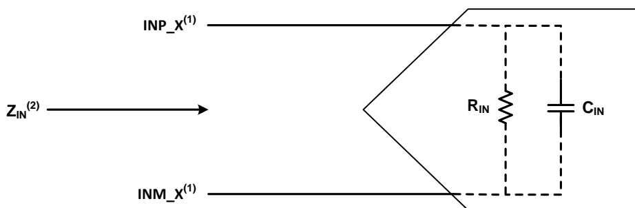
Figure 54. ADC Equivalent Input Impedance
