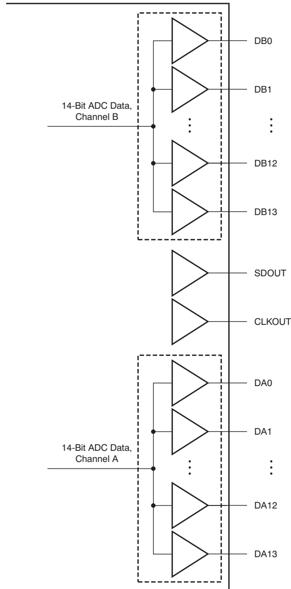
Figure 47. CMOS Outputs
