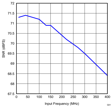
Figure 11. Signal-to-Noise Ratio vs Input Frequency
