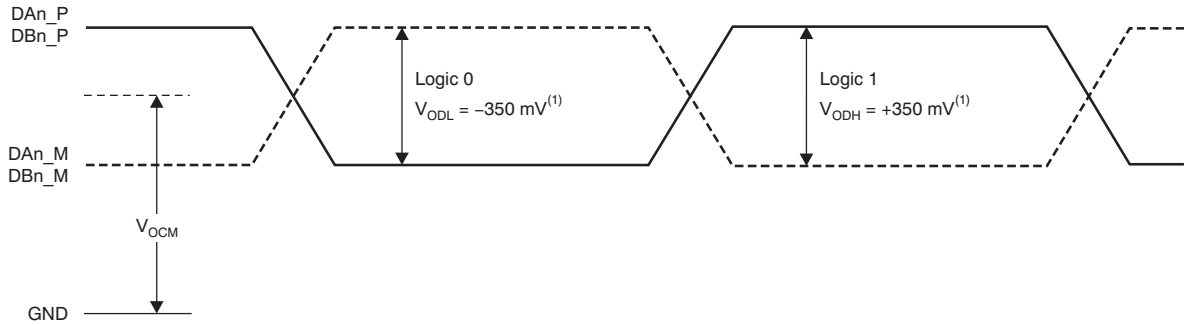
Figure 37. LVDS Output Voltage Levels
