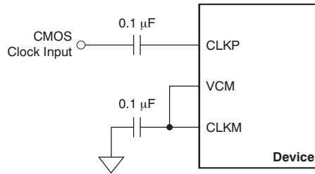
Figure 61. Single-Ended Clock Driving Circuit
