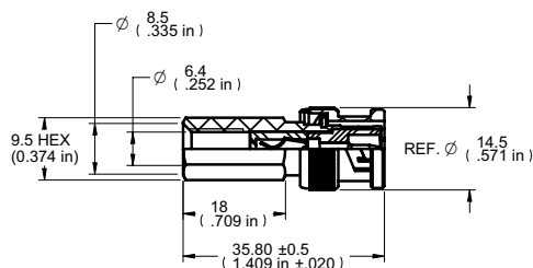
DIM OUTLINE
