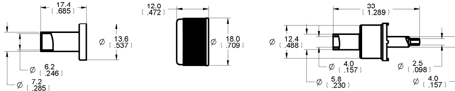
DIM OUTLINE
