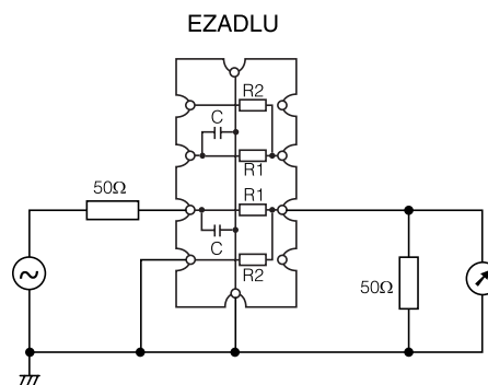
Measurement Circuit
