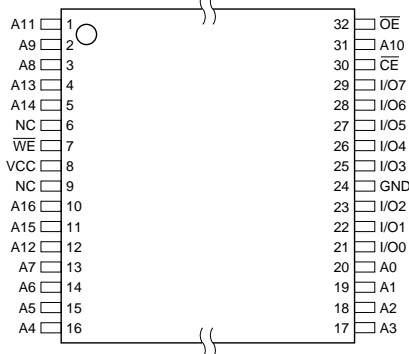
TSOP Top View
