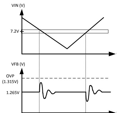
The Feedback Voltage Experiences an Oscillation if the Input Voltage Crosses the 7.2V Internal Bias Threshold
