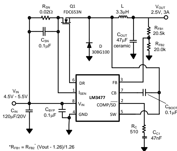
Figure 1. Typical High Efficiency Step-Down (Buck) Converter
