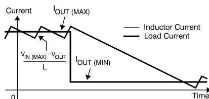
Figure 28. A Loading Transient
