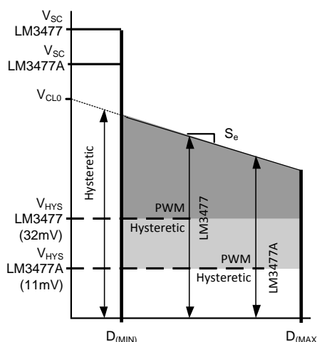
Figure 19. Operating Regions of the LM3477/A
