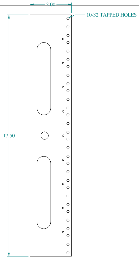
FRONT VIEW
