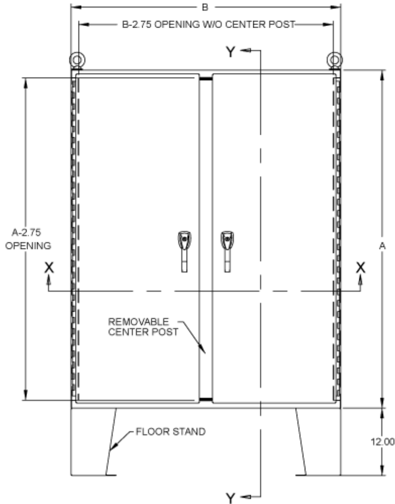
FRONT VIEW
