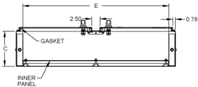
SECTION X-X
