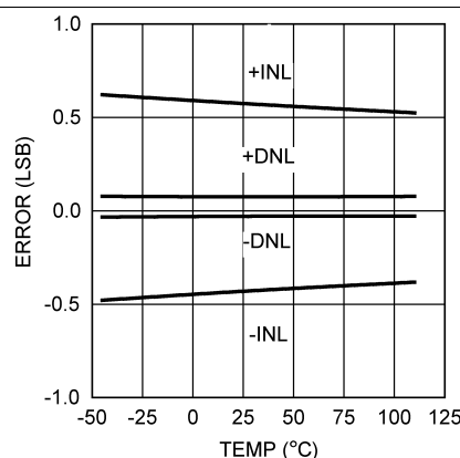
Figure 13. INL/DNL vs Temperature at V_A = 5 V
