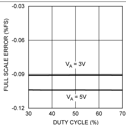
Figure 22. Full-Scale Error vs Clock Duty Cycle
