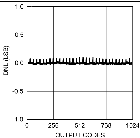
Figure 4. DNL at V_A = 3 V
