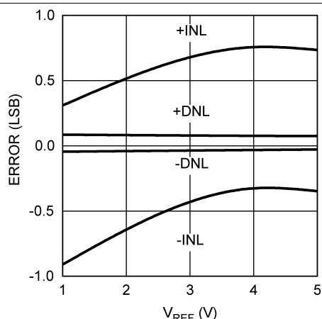
Figure 7. INL/DNL vs V_{REFIN} at V_A = 5 V
