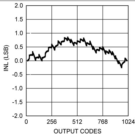
Figure 3. INL at V_A = 5 V
