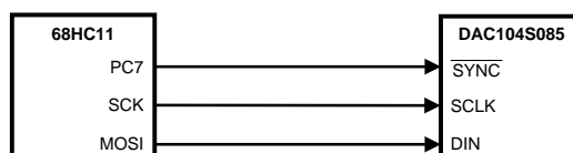
Figure 31. 68HC11 Interface
