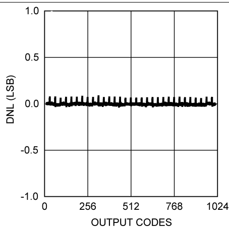
Figure 5. DNL at V_A = 5 V
