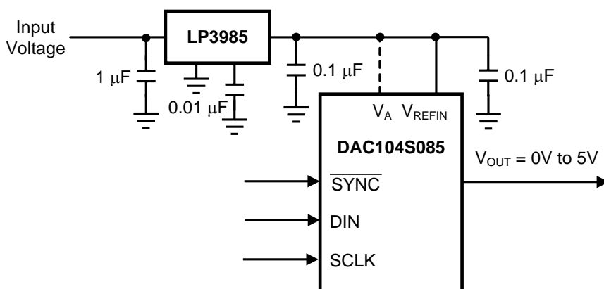
Figure 34. Using the LP3985 Regulator
