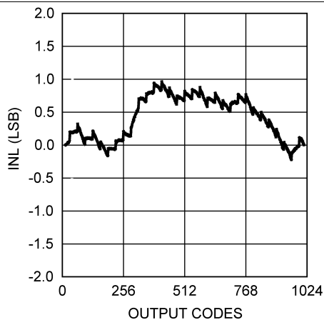
Figure 2. INL at V_A = 3 V
