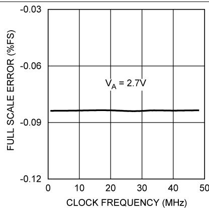
Figure 21. Full-Scale Error vs f_{SCLK}
