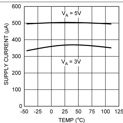
Figure 25. Supply Current vs Temperature
