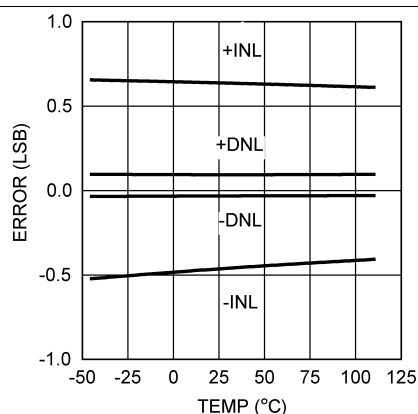
Figure 12. INL/DNL vs Temperature at V_A = 3 V
