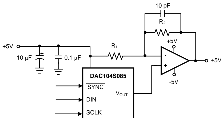
Figure 27. Bipolar Operation
