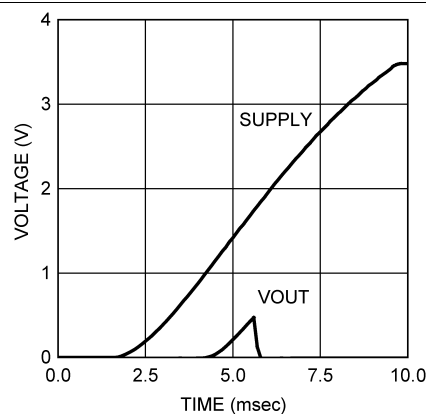
Figure 38. Power-On Reset
