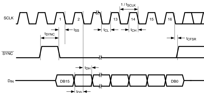
Figure 1. Serial Timing Diagram
