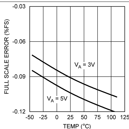
Figure 23. Full-Scale Error vs Temperature
