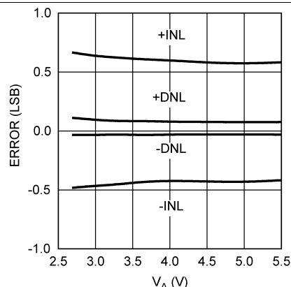
Figure 9. INL/DNL vs V_A
