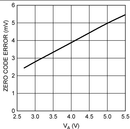
Figure 14. Zero Code Error vs V_A
