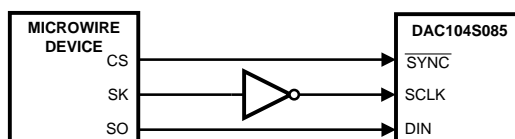
Figure 32. Microwire Interface
