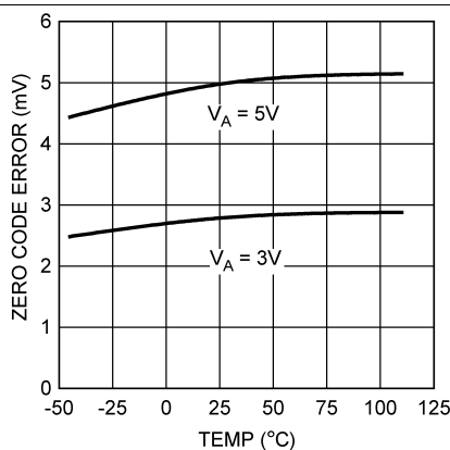
Figure 18. Zero Code Error vs Temperature
