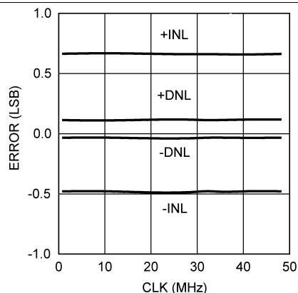
Figure 8. INL/DNL vs f_{SCLK} at V_A = 2.7 V
