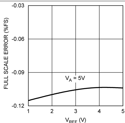
Figure 20. Full-Scale Error vs V_{REF}
