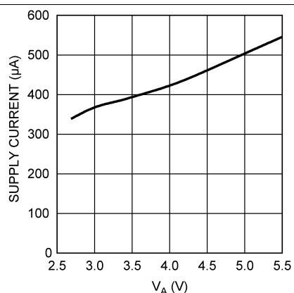
Figure 24. Supply Current vs V_A
