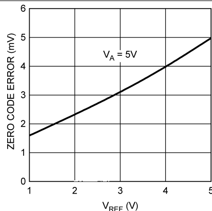
Figure 15. Zero Code Error vs. V_{REFIN}
