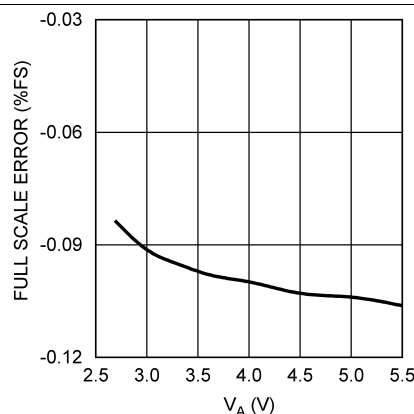
Figure 19. Full-Scale Error vs V_A
