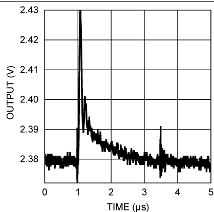
Figure 37. 5-V Glitch Response
