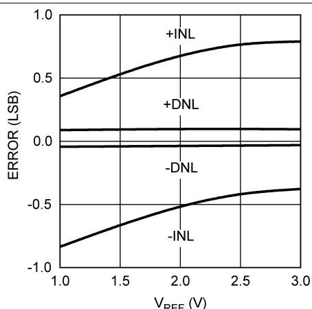
Figure 6. INL/DNL vs V_{REFIN} at V_A = 3 V
