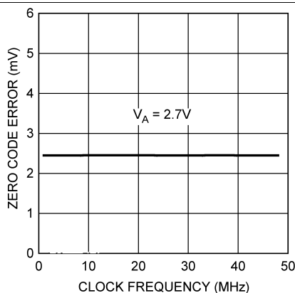
Figure 16. Zero Code Error vs f_{SCLK}
