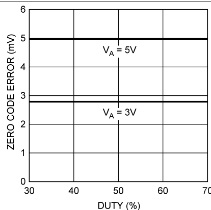
Figure 17. Zero Code Error vs Clock Duty Cycle
