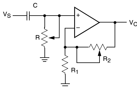
Filter
