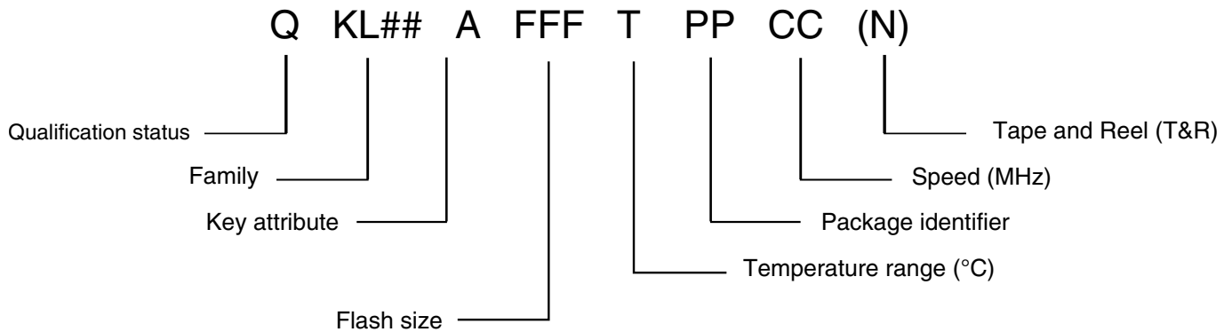
Figure 5. Part numbers diagrams
