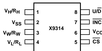
X9314 8 LD MSOP TOP VIEW
