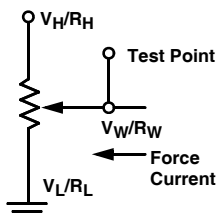
Test Circuit #2
