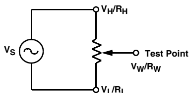
Test Circuit #1
