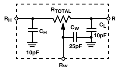
Circuit #3 SPICE Macro Model
