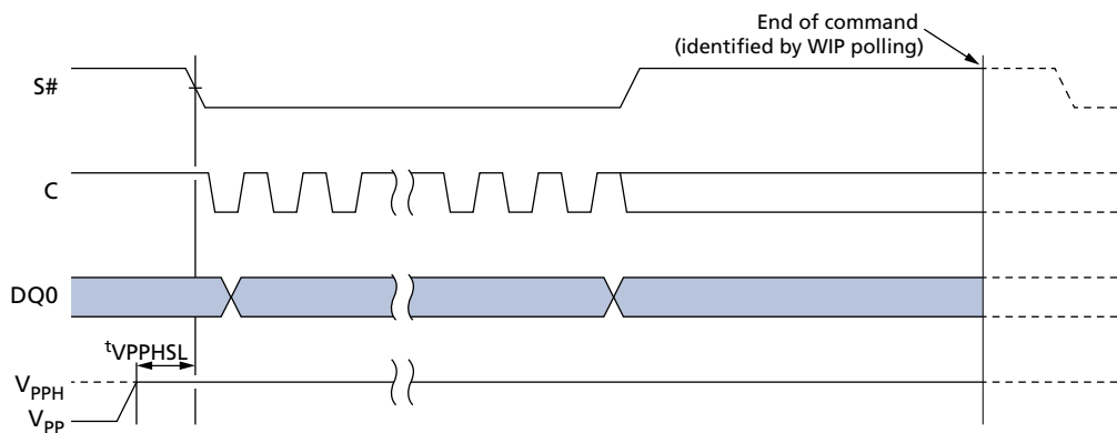
Figure 39: V_{PPH} Timing
