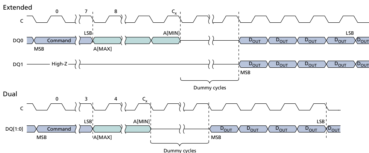
Figure 16: DUAL OUTPUT FAST READ
