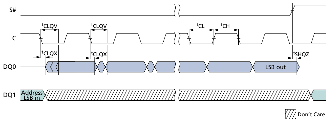
Figure 38: Output Timing
