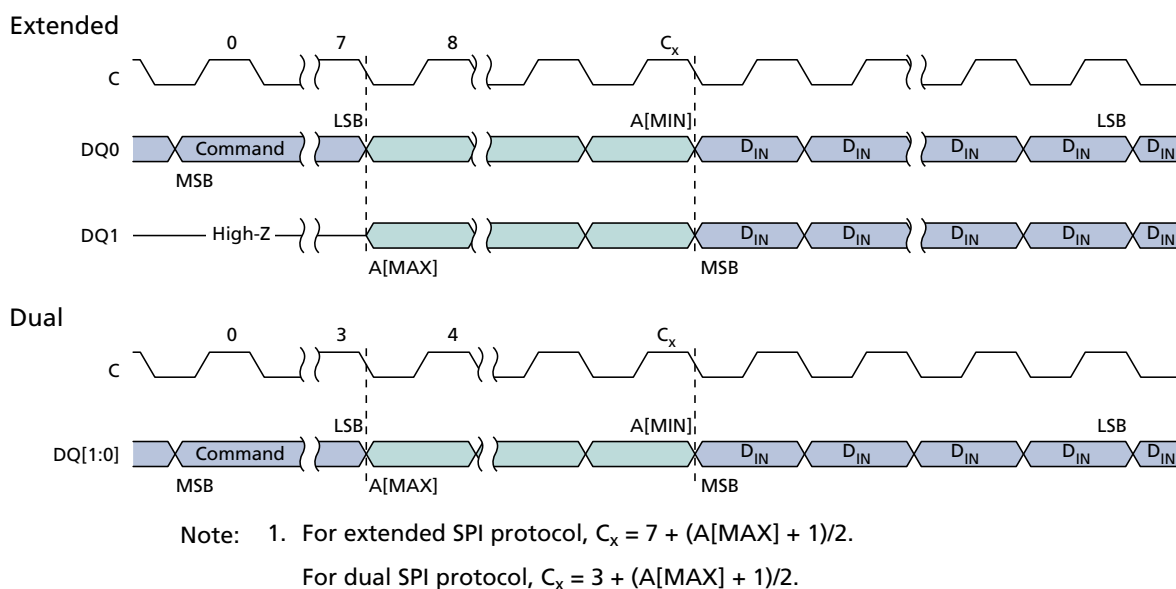
Figure 22: EXTENDED DUAL INPUT FAST PROGRAM Command
