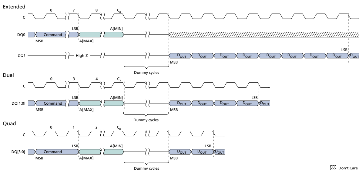
Figure 29: READ OTP Command
