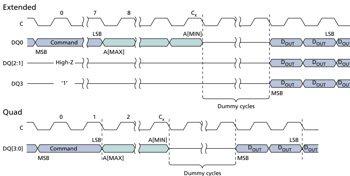
Figure 18: QUAD OUTPUT FAST READ Command
