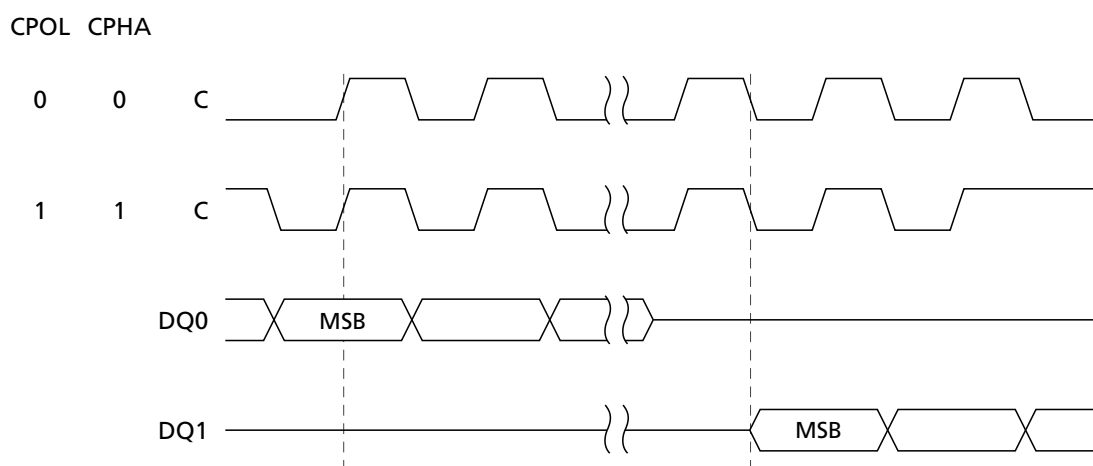
Figure 7: SPI Modes
