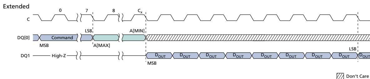
Figure 14: READ Command
