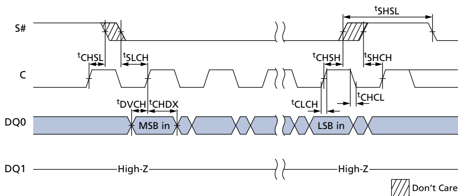
Figure 35: Serial Input Timing
