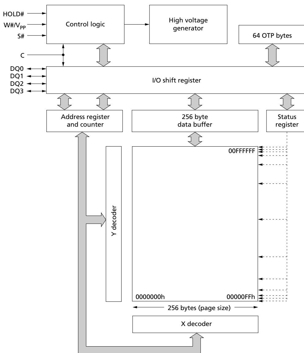
Figure 5: Block Diagram
