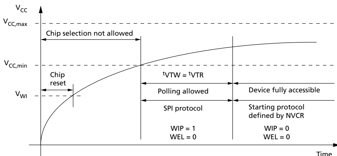
Figure 32: Power-Up Timing
