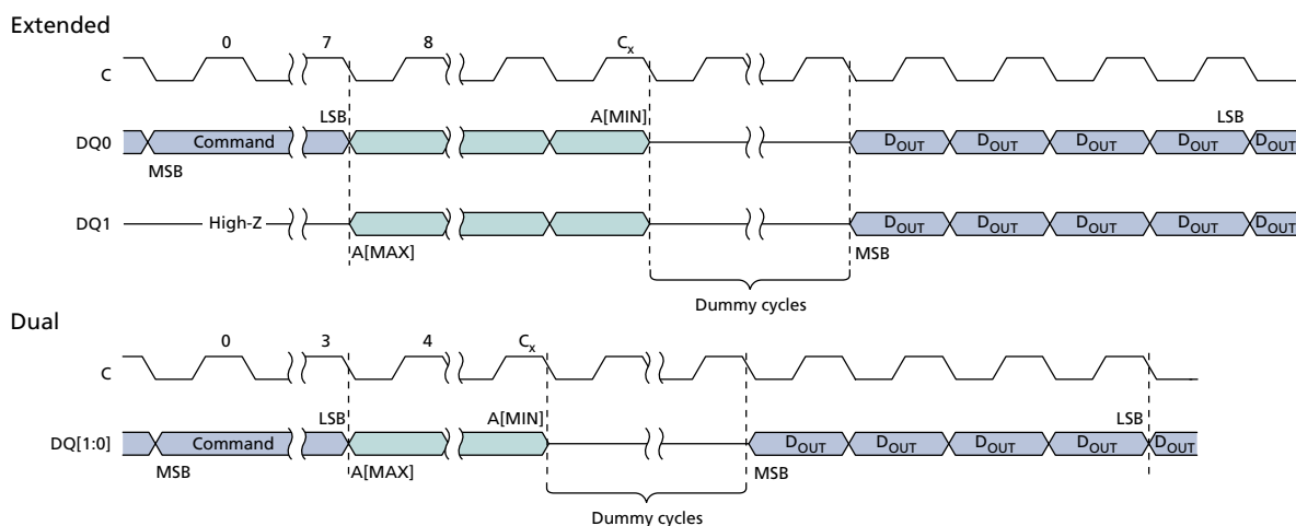
Figure 17: DUAL INPUT/OUTPUT FAST READ Command
