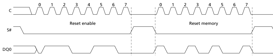
Figure 28: RESET ENABLE and RESET MEMORY Command
