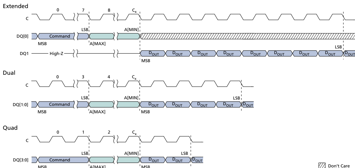
Figure 11: READ LOCK REGISTER Command
