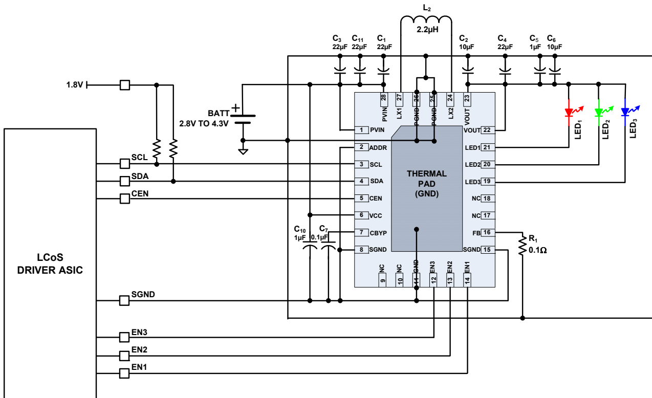
FIGURE 1. TYPICAL APPLICATION
