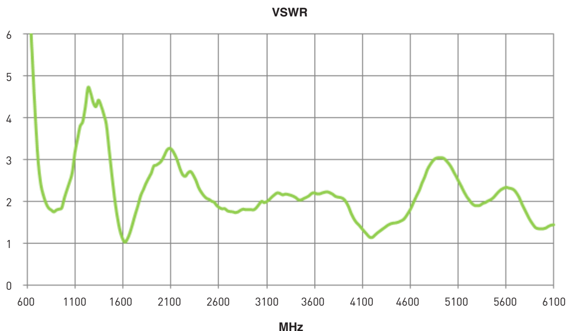
Figure 3. VSWR of FXUB66 UWB Antenna
