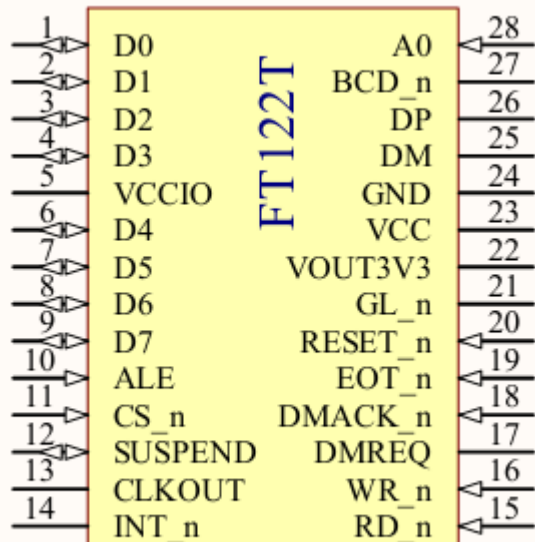
Figure 3-1 TSSOP-28 package schematic symbol
