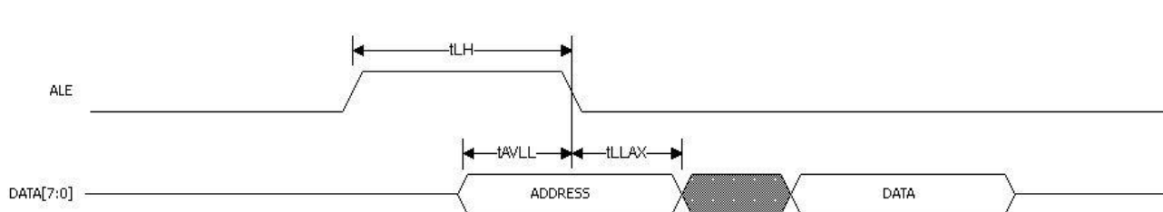
Figure 8-1 ALE Timing
