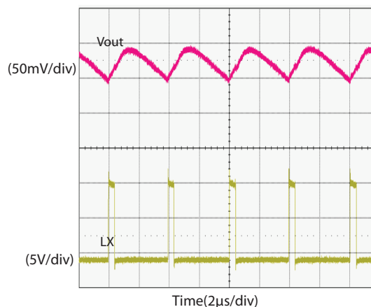
Forced Continuous Mode - No Load V_{IN} = 12\text{ V} , V_{OUT} = 1.2\text{ V} , I_{OUT} = 0\text{ A} , V_{DD} = EN/PSV = ENL = 5\text{ V}
