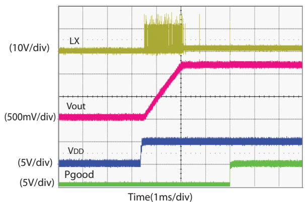
Self-Biased Start-Up - Power Good True V_{IN} = 12\text{ V} step, V_{OUT} = 1.2\text{ V} , I_{OUT} = 0\text{ A} , V_{DD} = EN/PSV = ENL = 5\text{ V}
