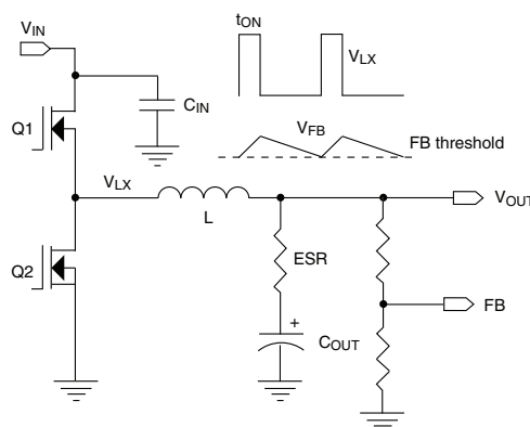
Fig. 1 - Output Ripple and PWM Control Method
