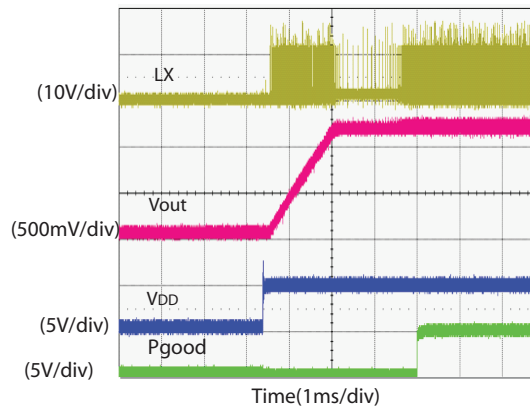
Enable Start-Up - Power Good True V_{IN} = 12\text{ V} , V_{OUT} = 1.2\text{ V} , I_{OUT} = 1\text{ A} , V_{DD} = EN/PSV = 5\text{ V}
