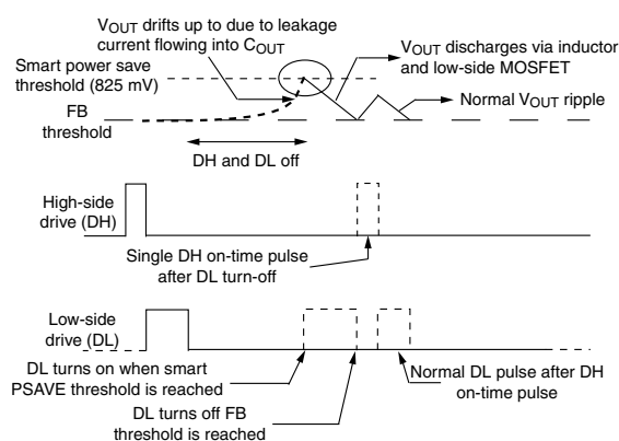
Fig. 7 - Smart Power-Save
