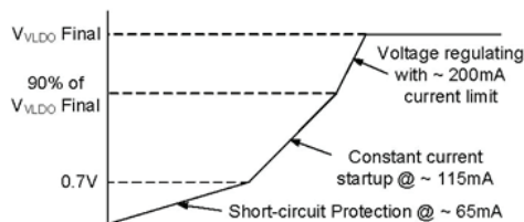
Fig. 11 - LDO Start-Up
