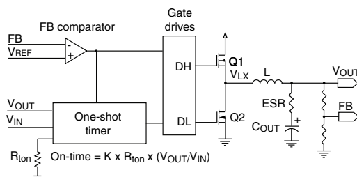
Fig. 2 - On-Time Generation
