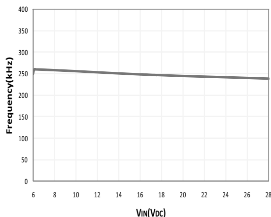
Frequency vs. Line-FCM Mode V OUT = 1.5 V, V LDO = V DD = ENL = 5 V, EN/PSV is Floating, SiC403B
