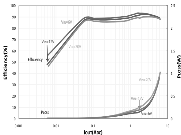
Efficiency vs. Load-PSAVE Mode V_{OUT} = 1.2\text{ V} , V_{DD} = 5\text{ V} = EN/PSV , External Bias, SiC403A
