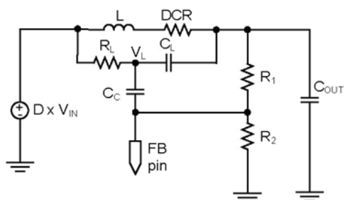
Fig. 14 - Virtual ESR Ramp Current
