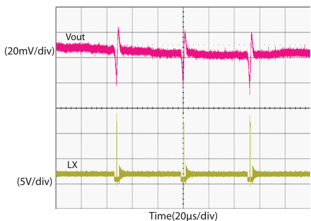
Powersave Mode - No Load V_{IN} = 12\text{ V} , V_{OUT} = 1.2\text{ V} , I_{OUT} = 0\text{ A} , V_{DD} = EN/PSV = ENL = 5\text{ V} , SiC403A
