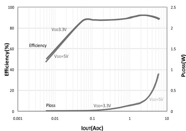
Efficiency vs. Load-PSAVE Mode V_{OUT} = 1.2\text{ V} , V_{IN} = 12\text{ V} , V_{DD} = EN/PSV = 5\text{ V} , External Bias, SiC403A
