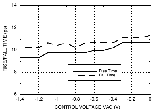
Rise / Fall Time vs. VAC [1][2][3]
