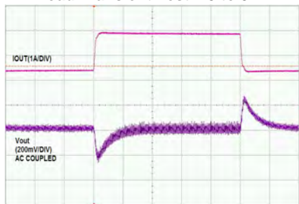
Load Transient Test 1.5 to 3A
