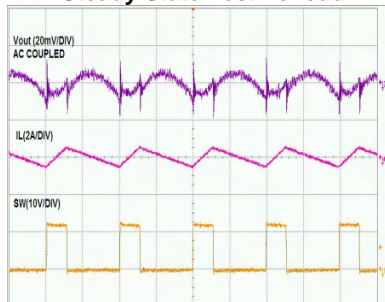
Steady State Test no load
