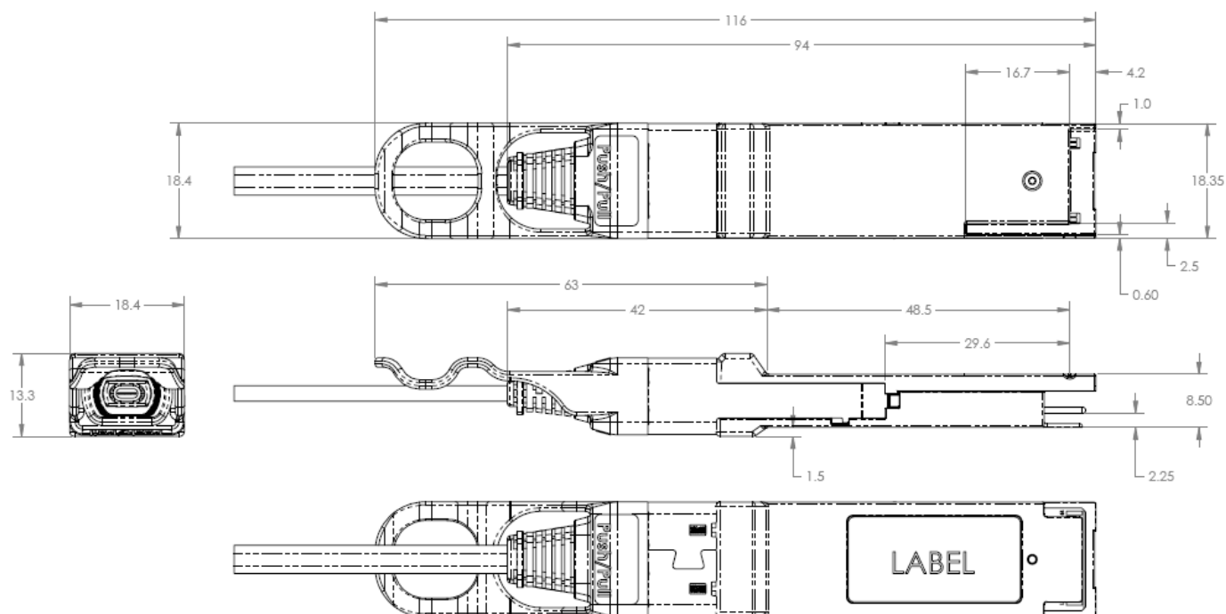
Figure 5 – Quadwire mechanical drawing
