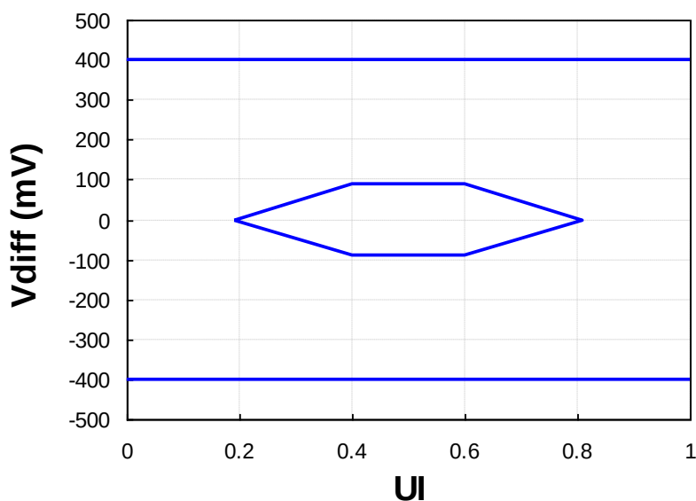
Figure 2 – Transmitter Input Differential Signal Mask
