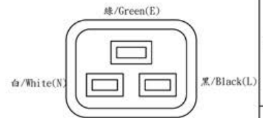
插頭端面圖 (Dimensions of Plug Face)
