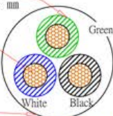
線材截面圖 (Wire Cross-Section)
