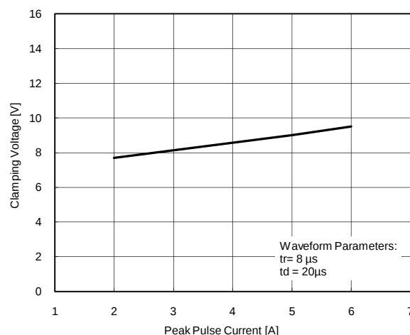
I/O Clamping Voltage vs. Peak Pulse Current
