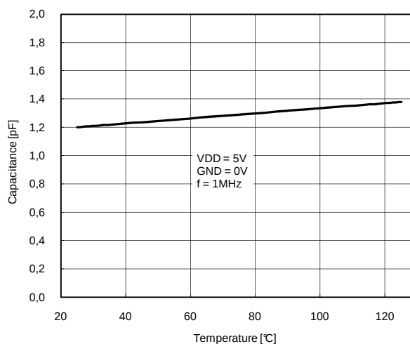
Variation of C_{IO} vs. Temp.
