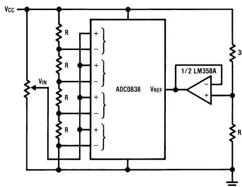
Figure 36. Obtaining Higher Resolution - 9-Bit A/D
