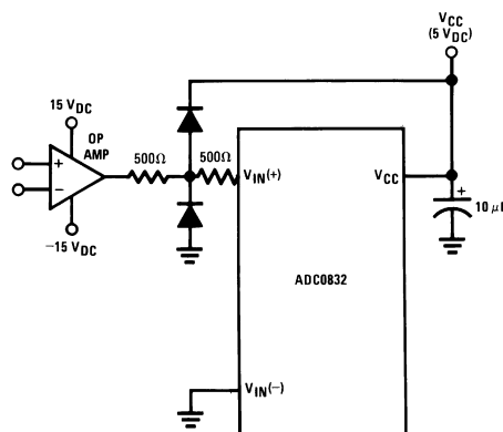
Figure 38. Protecting the Input
