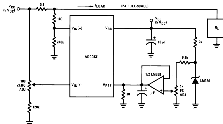
Figure 32. Digitizing a Current Flow
