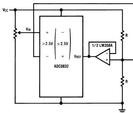
Figure 36. Obtaining Higher Resolution - 9-Bit A/D
