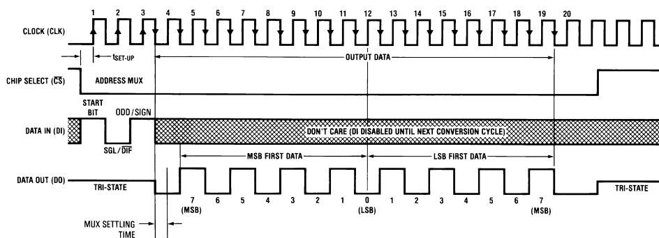
Figure 19. ADC0832-N Timing
