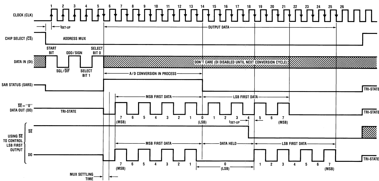
Figure 21. ADC0838-N Timing
