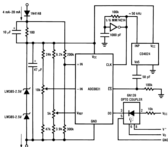
Figure 40. Digital Load Cell
