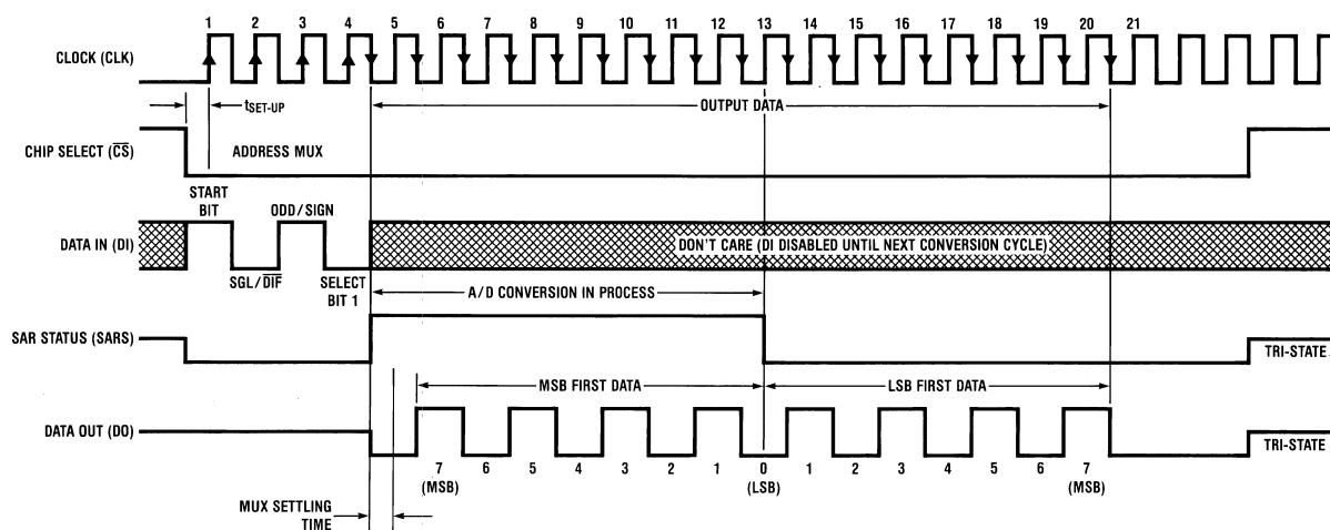
Figure 20. ADC0834-N Timing
