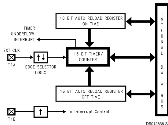
FIGURE 16. Timer in External Event Counter Mode
