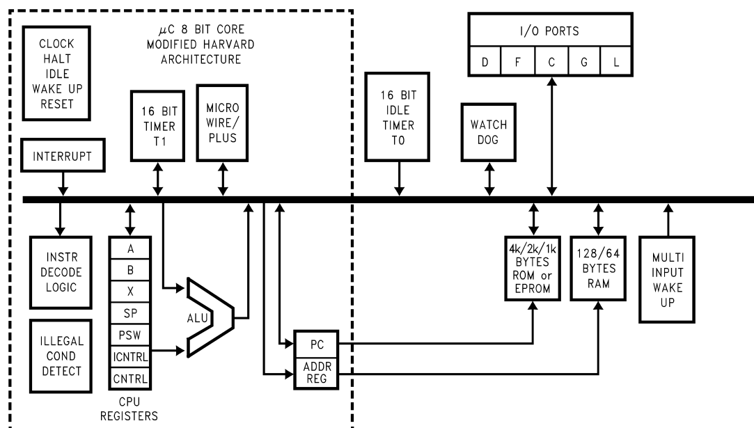
FIGURE 1. COP8SAx Block Diagram
