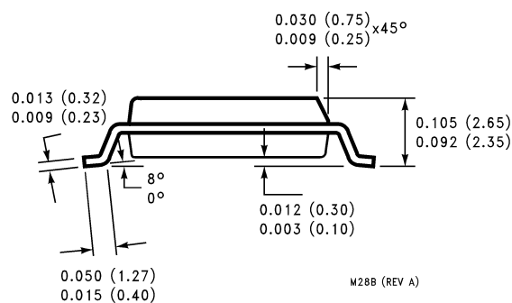
Molded SO Wide Body Package (WM) Order Number COP8SAA728M9, COP8SAB728M9, COP8SAC728M9, COP8SAA728M8, COP8SAB728M8 or COP8SAC728M8 NS Package Number M28B
