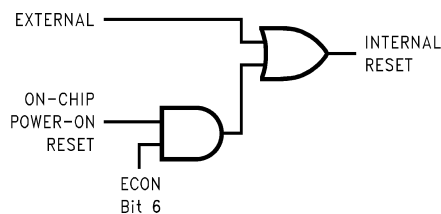
FIGURE 8. Reset Logic
