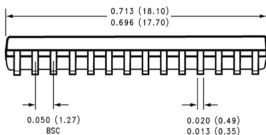
Molded SO Wide Body Package (WM) Order Number COP8SAA728M9, COP8SAB728M9, COP8SAC728M9, COP8SAA728M8, COP8SAB728M8 or COP8SAC728M8 NS Package Number M28B
