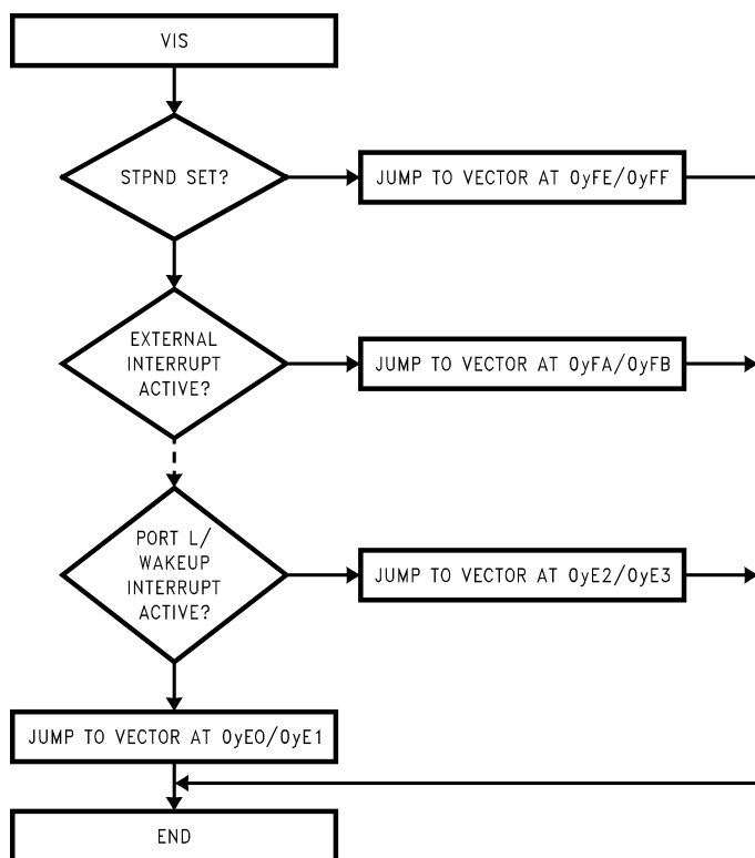
FIGURE 23. VIS Flowchart
