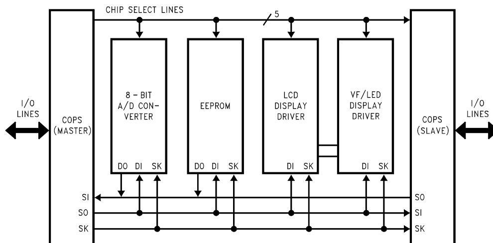
FIGURE 24. MICROWIRE/PLUS Application
