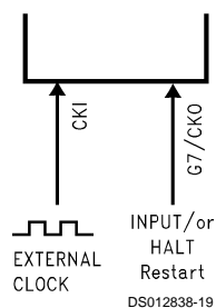
FIGURE 13. External Oscillator
