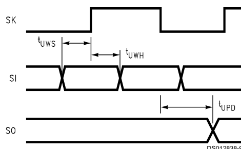
FIGURE 4. MICROWIRE/PLUS Timing
