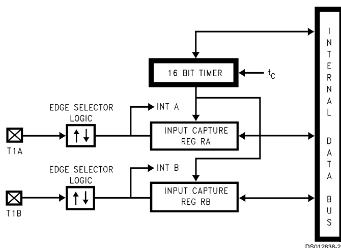
FIGURE 17. Timer in Input Capture Mode
