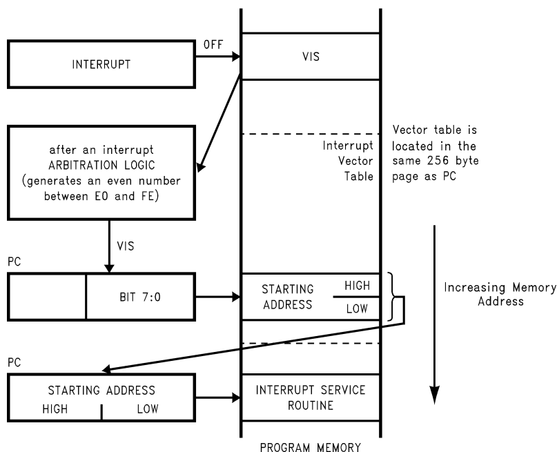
Figure 5-21. VIS Operation
