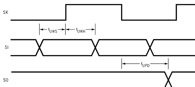
Figure 3-1. MICROWIRE/PLUS Timing
