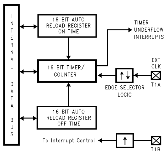
Figure 5-11. Timer in External Event Counter Mode
