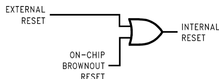
Figure 5-2. Reset Logic
