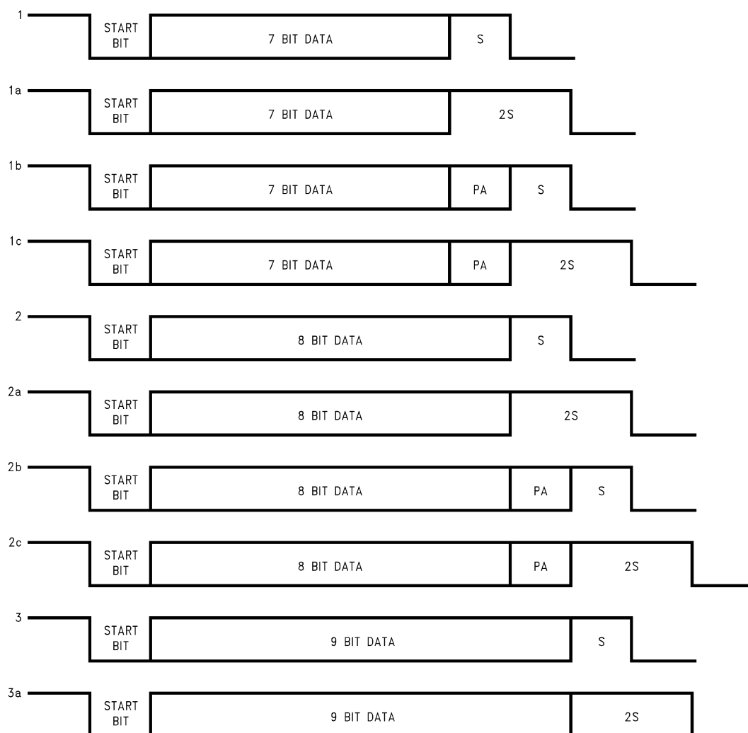
Figure 5-17. Framing Formats
