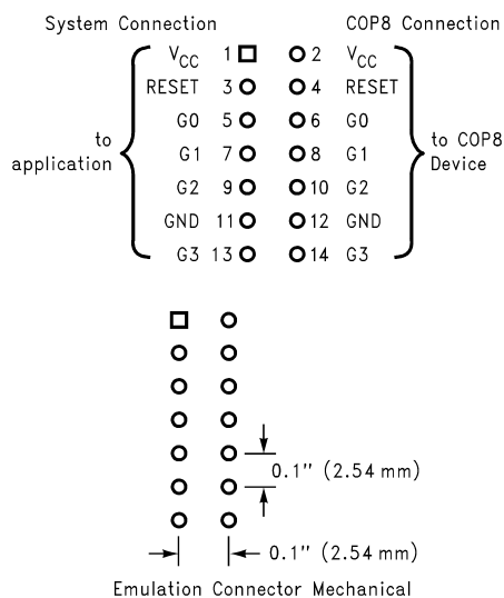
Figure 4-5. Emulation Connection
