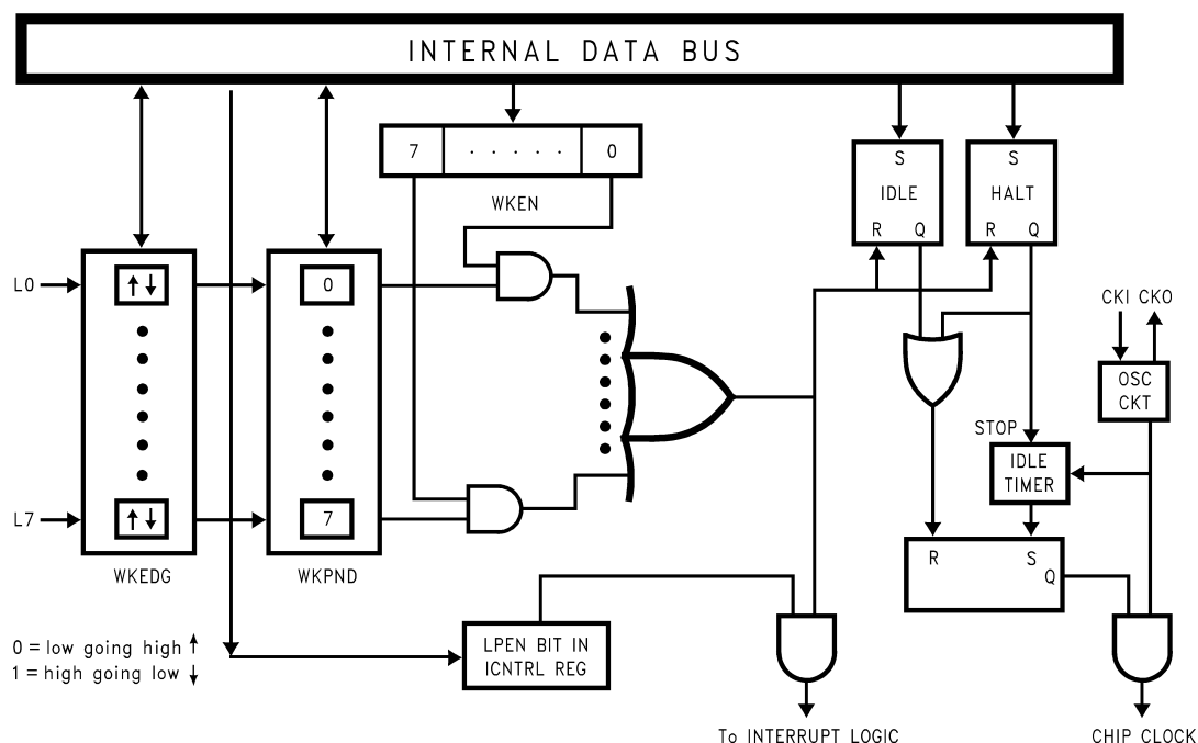
Figure 5-15. Multi-Input Wake-Up Logic
