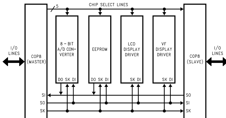
Figure 5-23. MICROWIRE/PLUS Application
