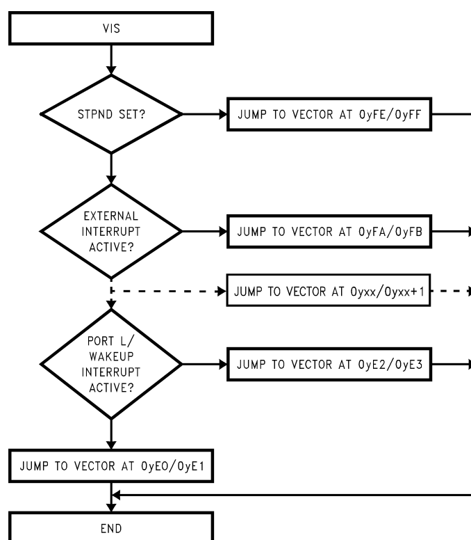
Figure 5-22. VIS Flow Chart
