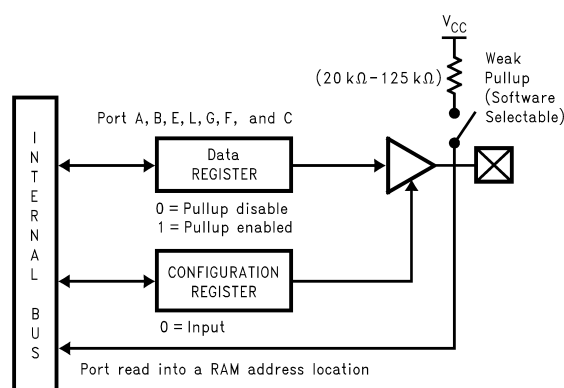
Figure 4-4. I/O Port Configurations—Input Mode
