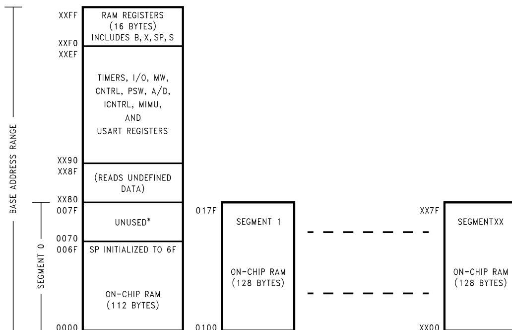
Figure 5-1. RAM Organization
