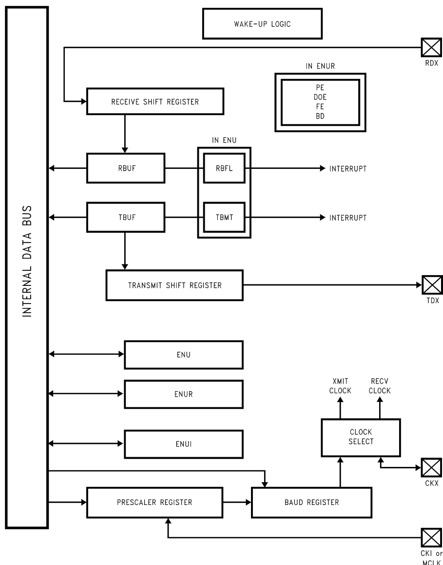
Figure 5-16. USART Block Diagram
