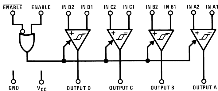
Logic Diagram
