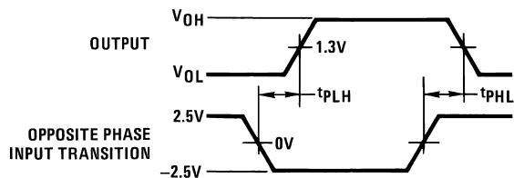
Figure 4. Propagation Delay
