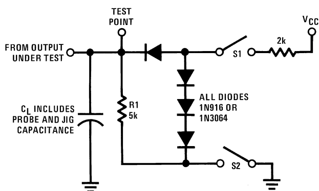
Figure 3. Load Test Circuit for TRI-STATE Outputs
