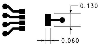
Figure 27. SCENARIO A, \theta_{JA} = 148^{\circ}\text{C/W}
