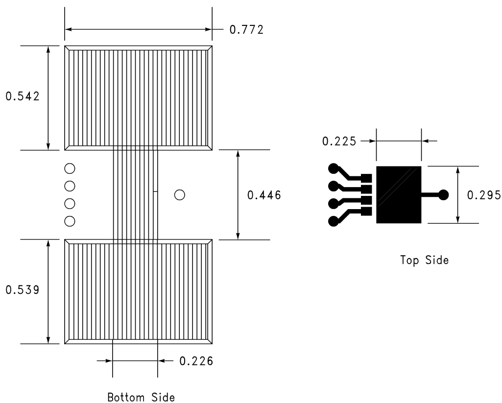
Figure 35. SCENARIO I, \theta_{JA} = 78.5^{\circ}\text{C/W}
