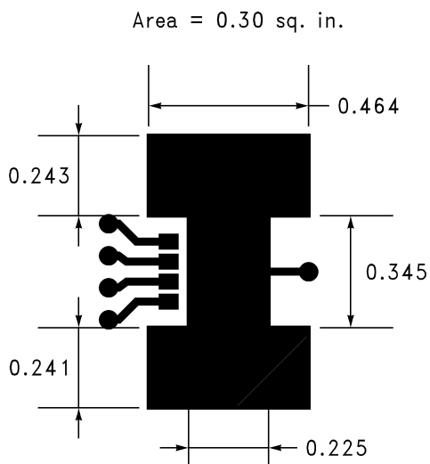
Figure 29. SCENARIO C, \theta_{JA} = 92^{\circ}\text{C/W}
