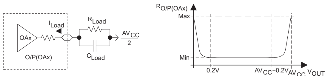
Figure 25. OAx Output Resistance Tests
