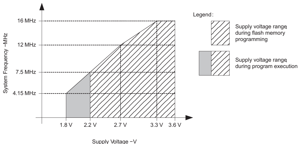
Figure 1. Operating Area
