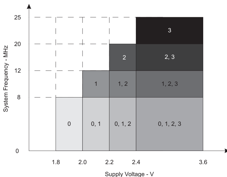
Figure 3. Maximum System Frequency
