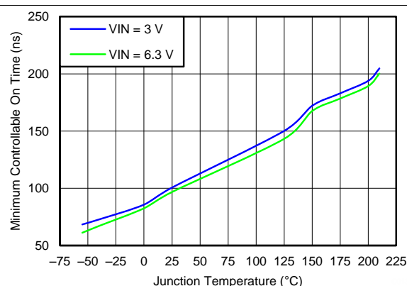
Figure 15. Minimum Controllable On-Time vs Temperature
