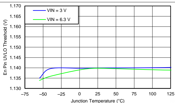
Figure 8. EN Pin UVLO Threshold vs Temperature
