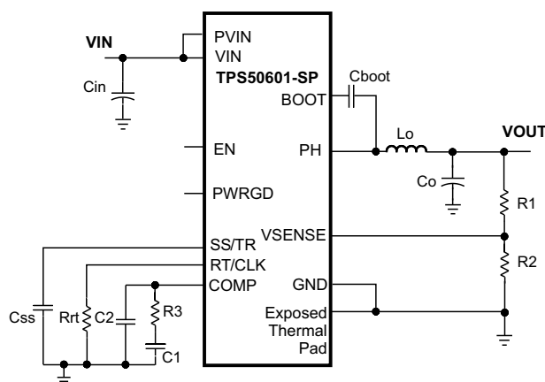
Figure 29. Typical Application Schematic
