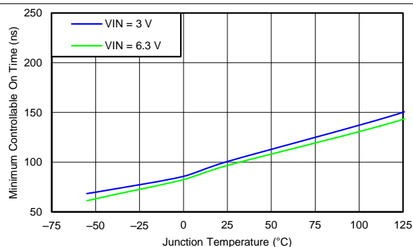
Figure 15. Minimum Controllable On-Time vs Temperature
