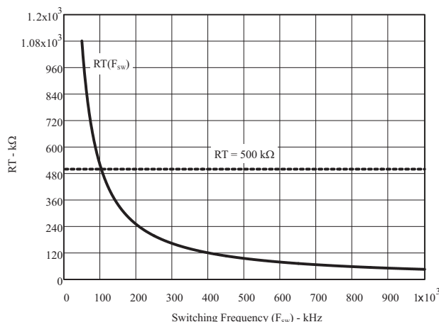
Figure 21. RT vs Switching Frequency
