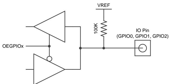
Figure 8. GPIO signals.
