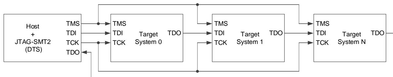
Figure 3. 4-Wire series topology.
