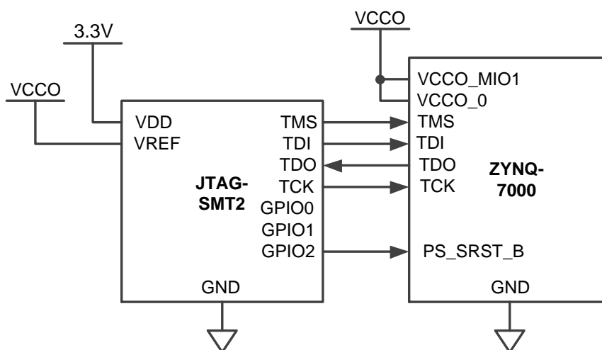
Figure 9. Connecting the JTAG-SMT2 to Xilinx's Zynq-7000.
