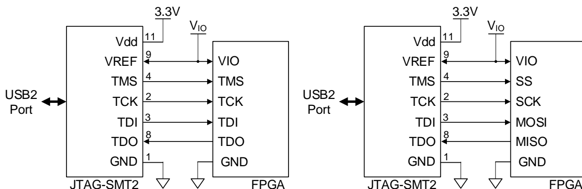
Figure 1. JTAG-SMT2 port connections.
