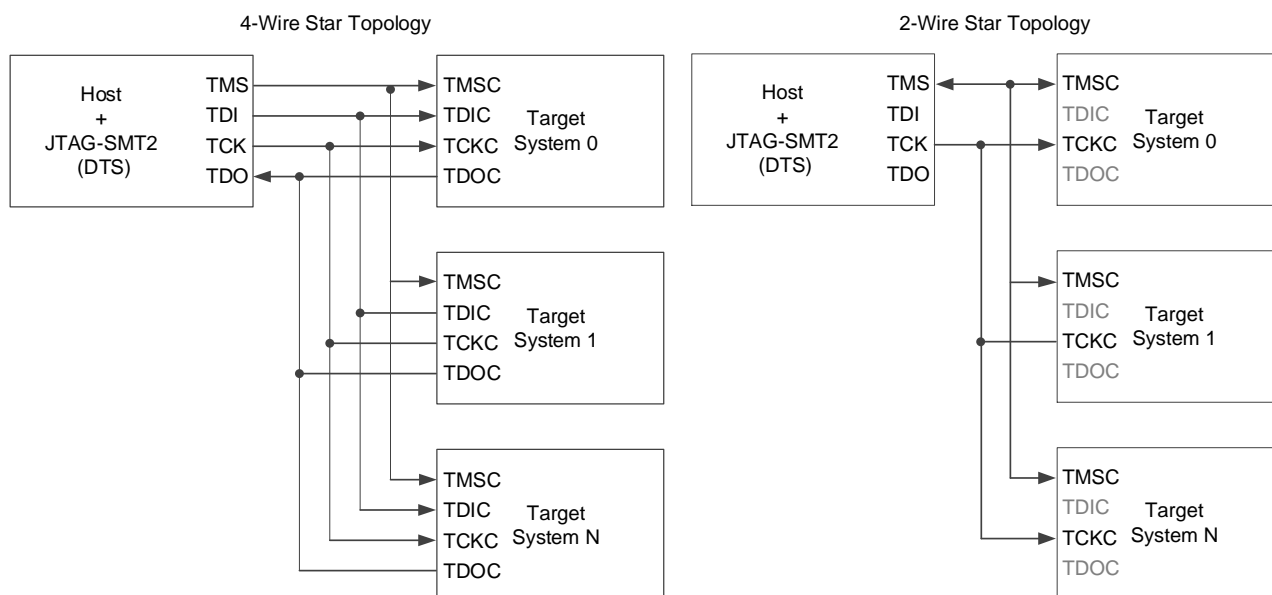
Figure 4. 4-Wire and 2-Wire star topology.
