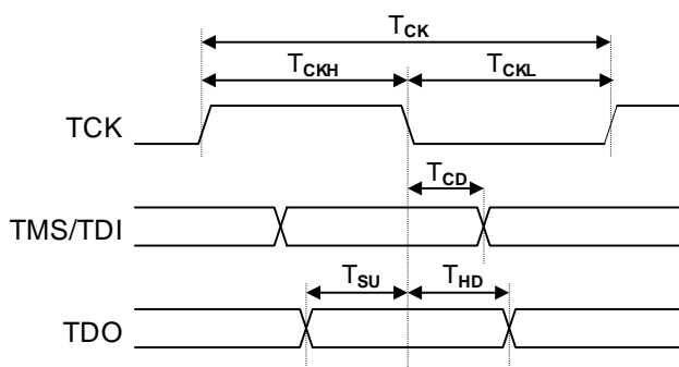
Figure 12. Timing diagram.
