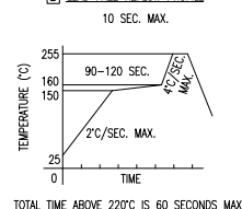
B LEAD FREE REFLOW PROFILE
