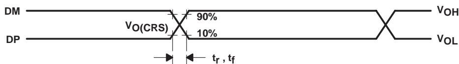
Figure 3-2. USB Differential Driver Timing Waveform
