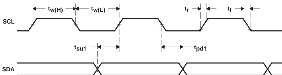
Figure 3-7. SCL and SDA Timing Waveforms
