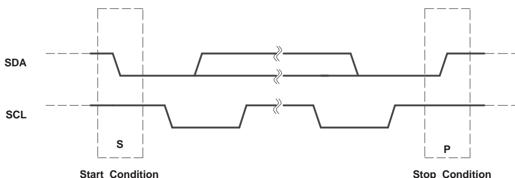
Figure 2–12. I 2 C START and STOP Conditions
