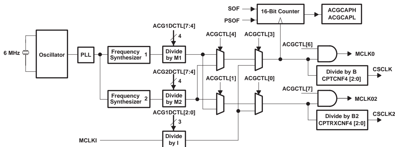
Figure 2–1. Adaptive Clock Generator
