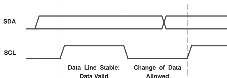
Figure 2–11. Bit Transfer on the I 2 C Bus
