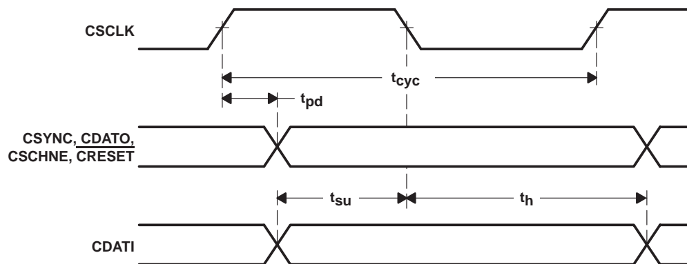
Figure 3-6. General-Purpose Mode Timing Waveforms
