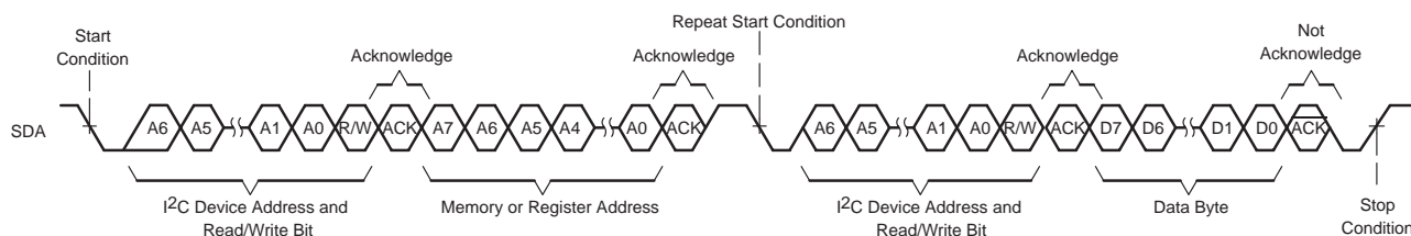
Figure 2–16. Single Byte Read Transfer
