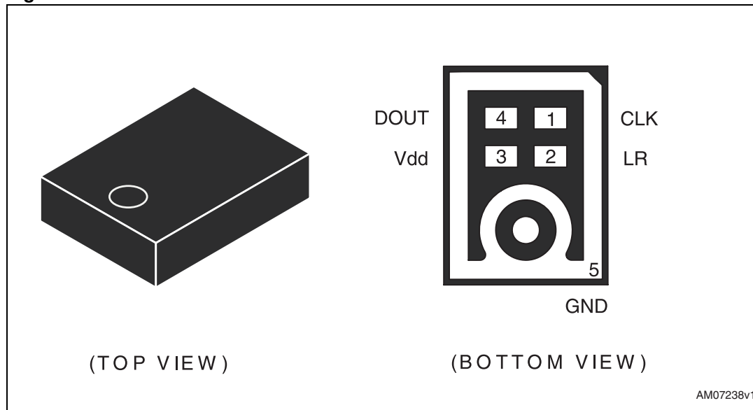
Figure 1. Pin connections
