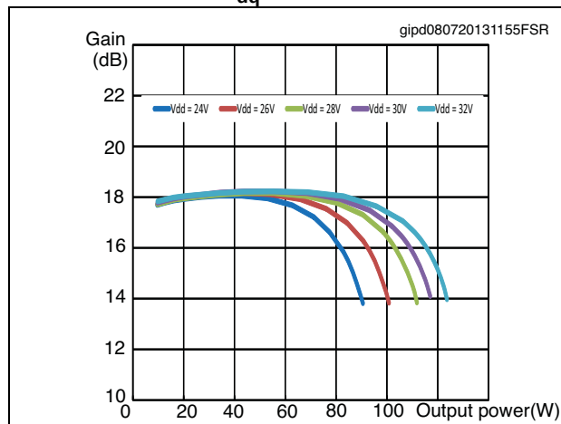
Figure 7. Gain vs output power, freq = 945 MHz, I_{dq} = 0.4 A
