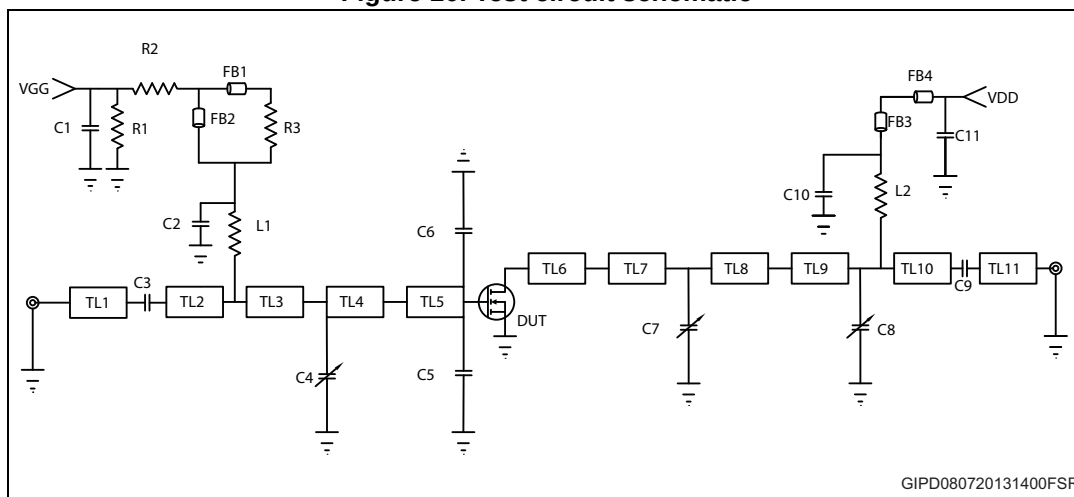
Figure 10. Test circuit schematic
