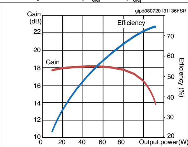
Figure 6. Gain and efficiency vs output power, freq = 945 MHz, V_{dd} = 28\text{ V} , I_{dq} = 0.4\text{ A}
