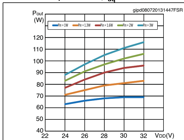
Figure 9. Output power vs supply voltage, freq = 945 MHz, I_{dq} = 0.4 A
