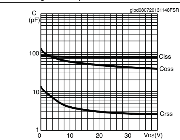
Figure 4. Capacitance variation
