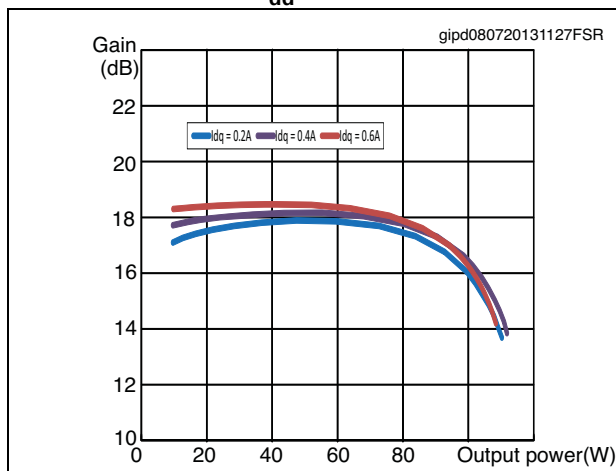
Figure 5. Gain vs output power, freq = 945 MHz, V_{dd} = 28\text{ V}
