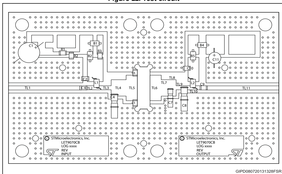
Figure 11. Test circuit
