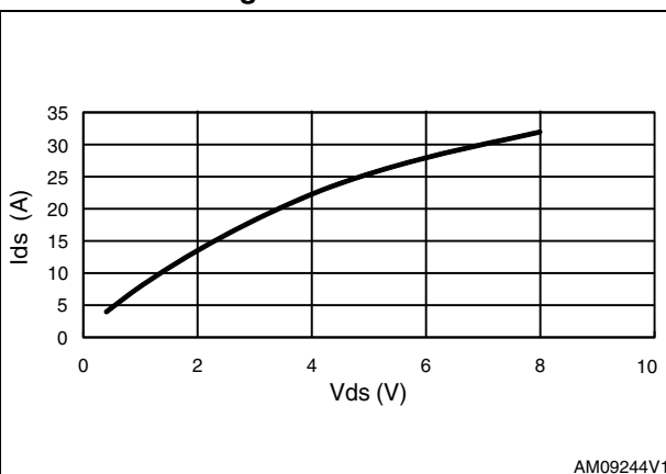
Figure 4. Drain current vs. drain-source voltage
